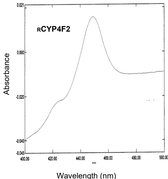
CO Reduced Difference Spectrum of Purified RCYP4F2
